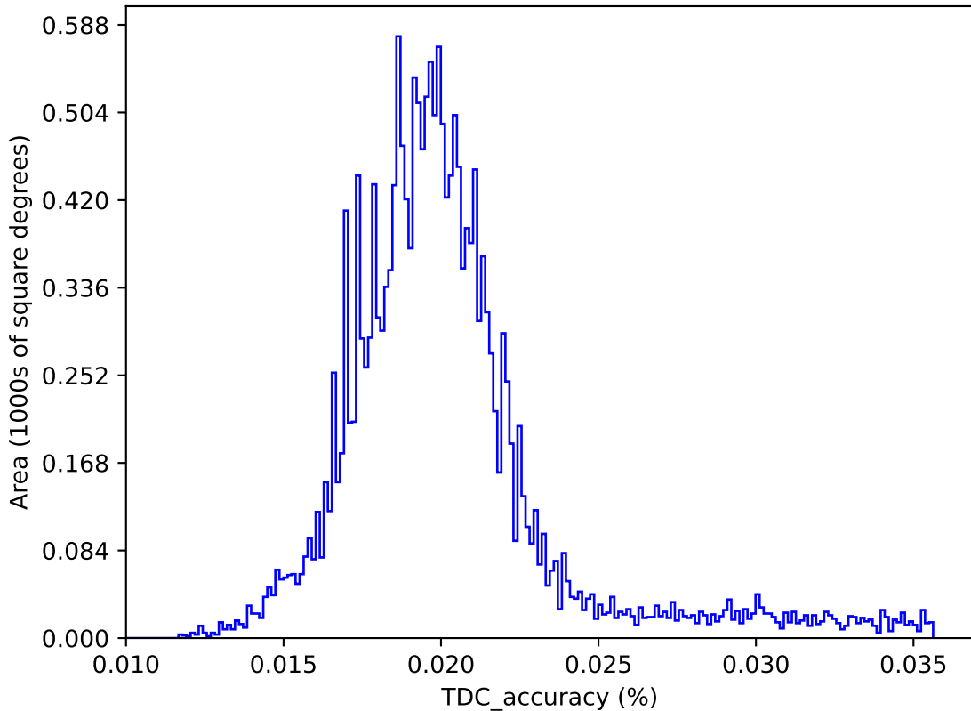
extra_ss_neo4_v3.4_10yrs : TDC_accuracy
