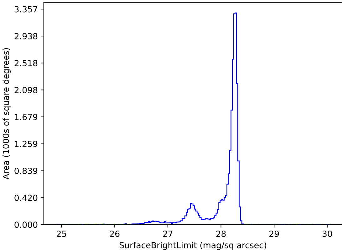
extra_ss_neo4_v3.4_10yrs y: SurfaceBrightLimit
