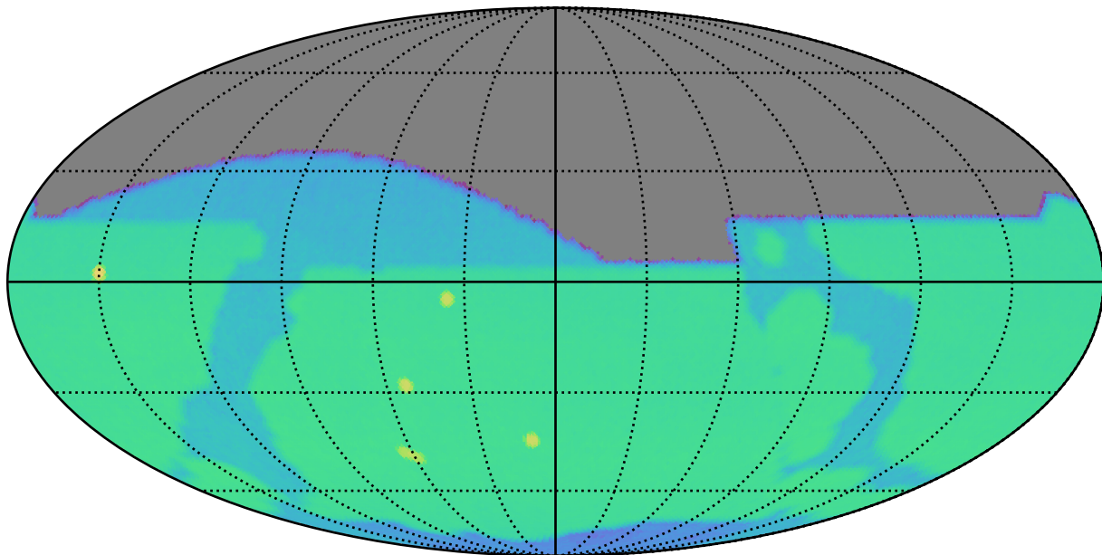
extra_ss_neo4_v3.4_10yrs r: SurfaceBrightLimit
