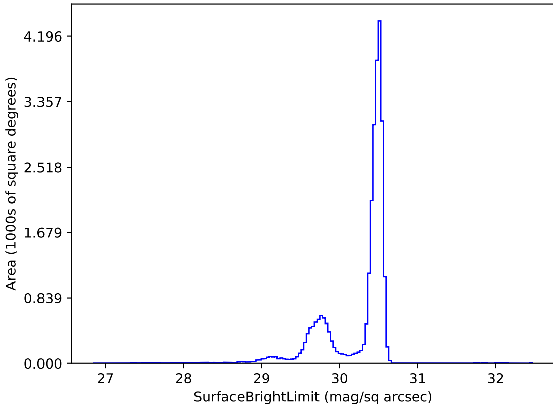
extra_ss_neo4_v3.4_10yrs r: SurfaceBrightLimit
