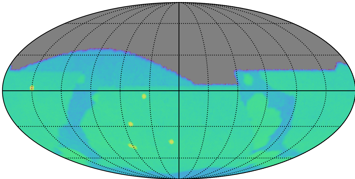
extra_ss_neo4_v3.4_10yrs g: SurfaceBrightLimit
