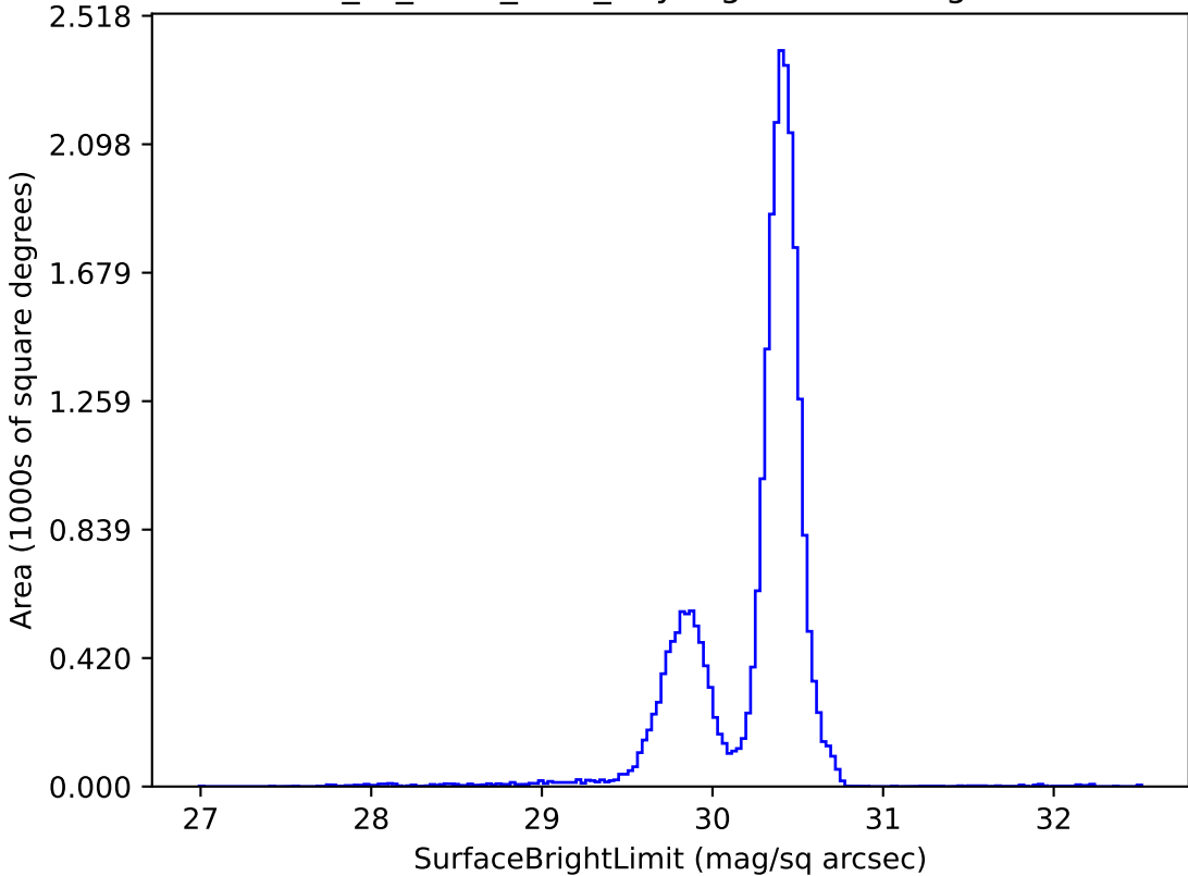
extra_ss_neo4_v3.4_10yrs g: SurfaceBrightLimit
