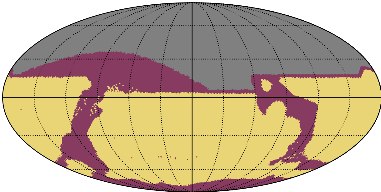
extra_ss_neo4_v3.4_10yrs : RapidRevisits
