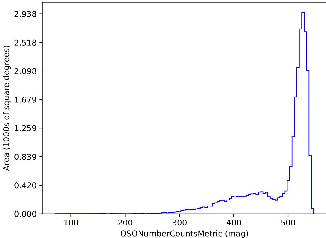
extra_ss_neo4_v3.4_10yrs r band and non-DD: QSONumberCountsMetric
