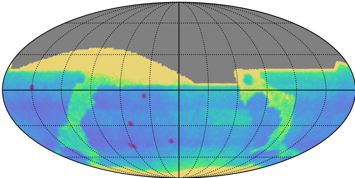
extra_ss_neo4_v3.4_10yrs : Proper Motion Uncert @ 24.0
