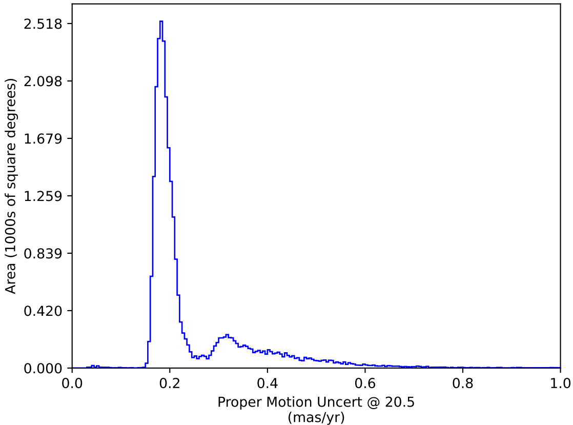
extra_ss_neo4_v3.4_10yrs : Proper Motion Uncert @ 20.5
