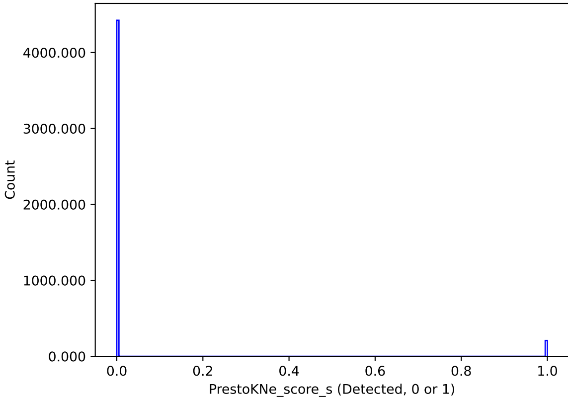
extra_ss_neo4_v3.4_10yrs : PrestoKNe_score_s
