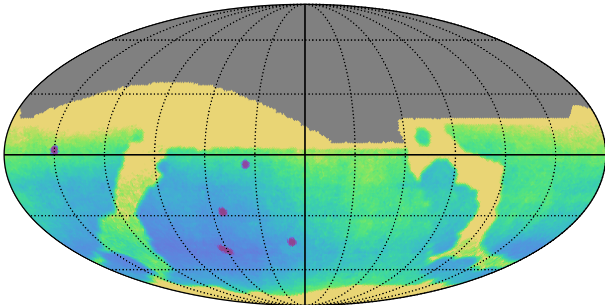
extra_ss_neo4_v3.4_10yrs : Parallax Uncert @ 24.0
