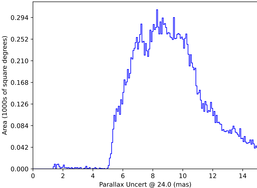
extra_ss_neo4_v3.4_10yrs : Parallax Uncert @ 24.0
