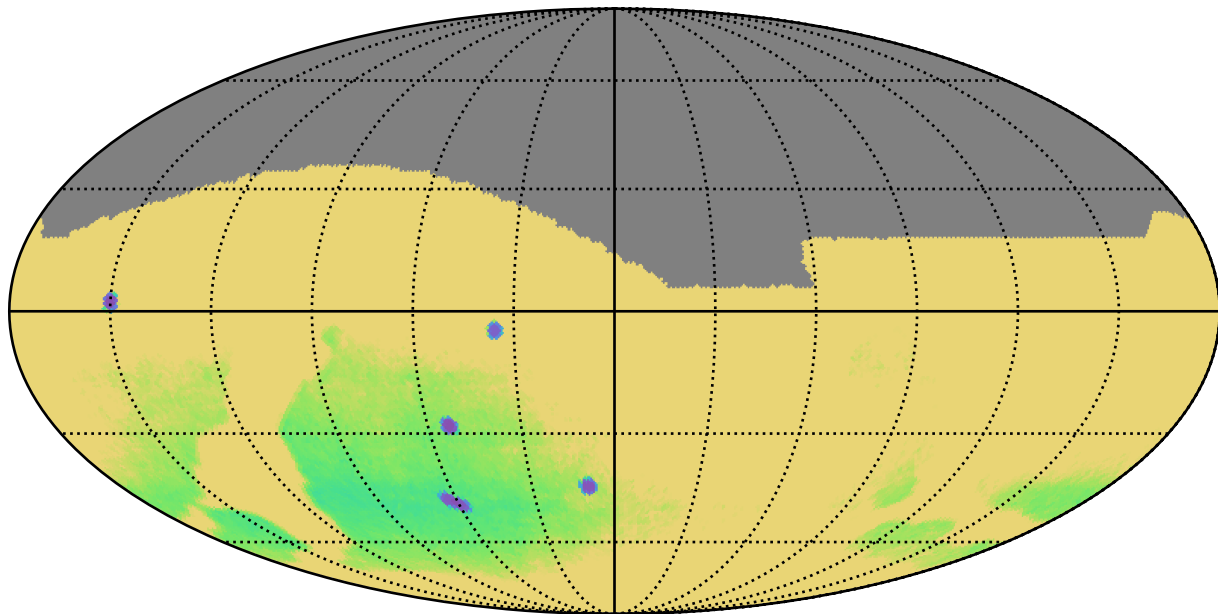
extra_ss_neo4_v3.4_10yrs : Parallax Uncert @ 22.4
