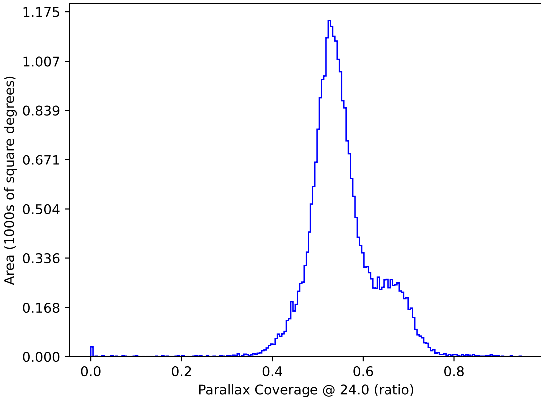
extra_ss_neo4_v3.4_10yrs : Parallax Coverage @ 24.0
