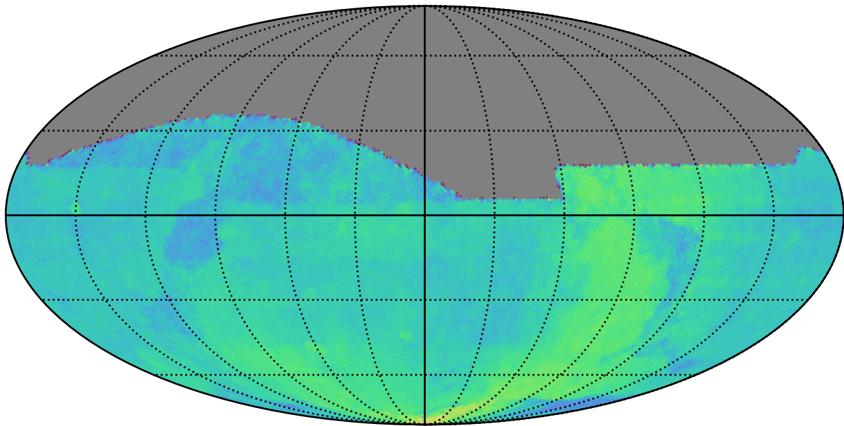
extra_ss_neo4_v3.4_10yrs : Parallax Coverage @ 22.4
