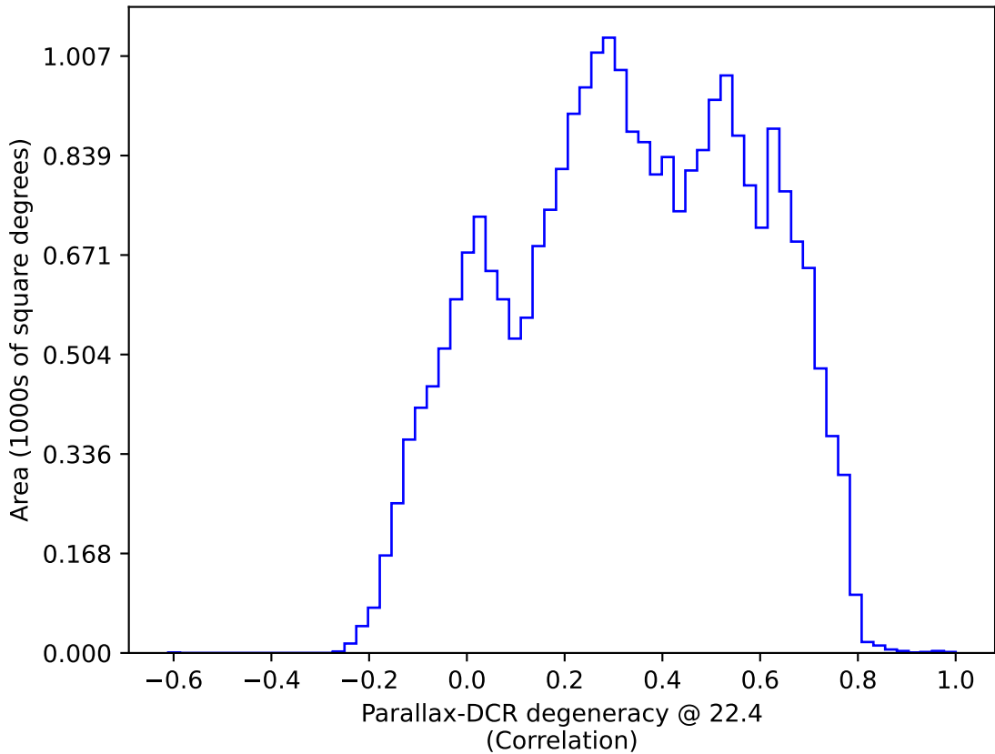
extra_ss_neo4_v3.4_10yrs : Parallax-DCR degeneracy @ 22.4
