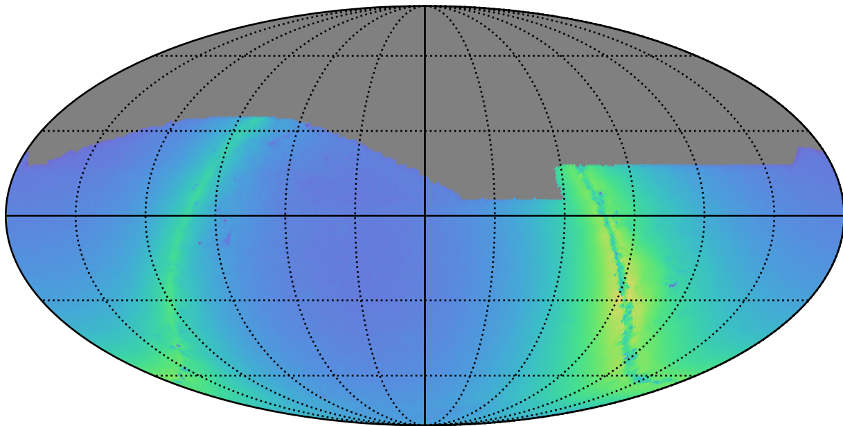
extra_ss_neo4_v3.4_10yrs r: Nstars_no_crowding
