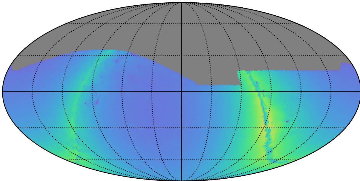
extra_ss_neo4_v3.4_10yrs g: Nstars_no_crowding
