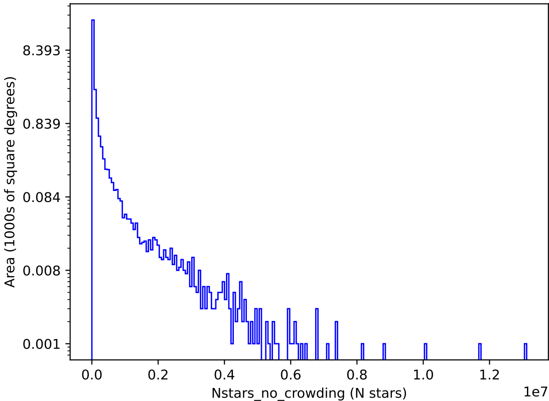
extra_ss_neo4_v3.4_10yrs g: Nstars_no_crowding
