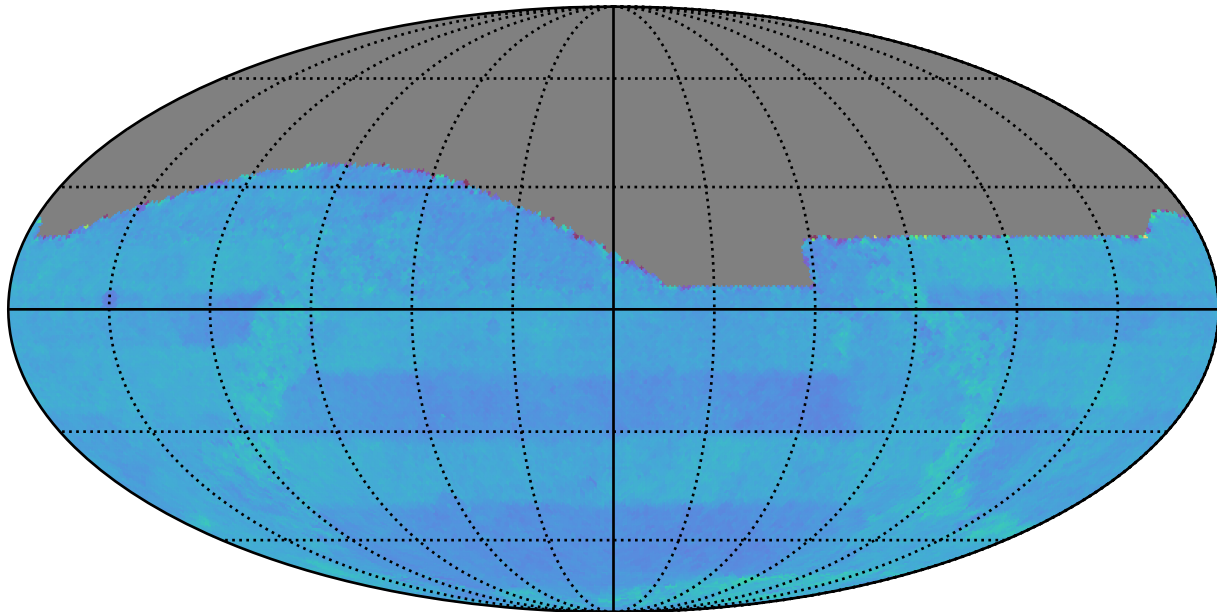
extra_ss_neo4_v3.4_10yrs : Normalized Proper Motion Uncert @ 24.0
