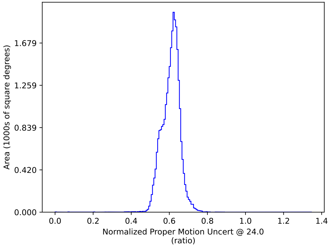
extra_ss_neo4_v3.4_10yrs : Normalized Proper Motion Uncert @ 24.0
