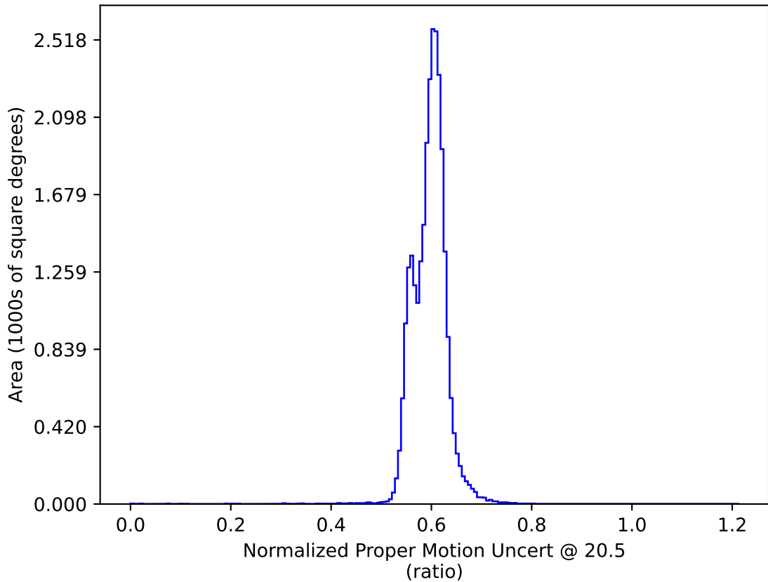
extra_ss_neo4_v3.4_10yrs : Normalized Proper Motion Uncert @ 20.5
