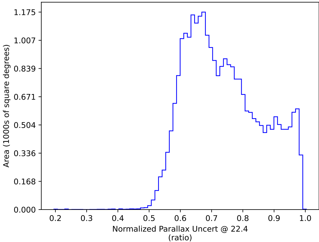
extra_ss_neo4_v3.4_10yrs : Normalized Parallax Uncert @ 22.4
