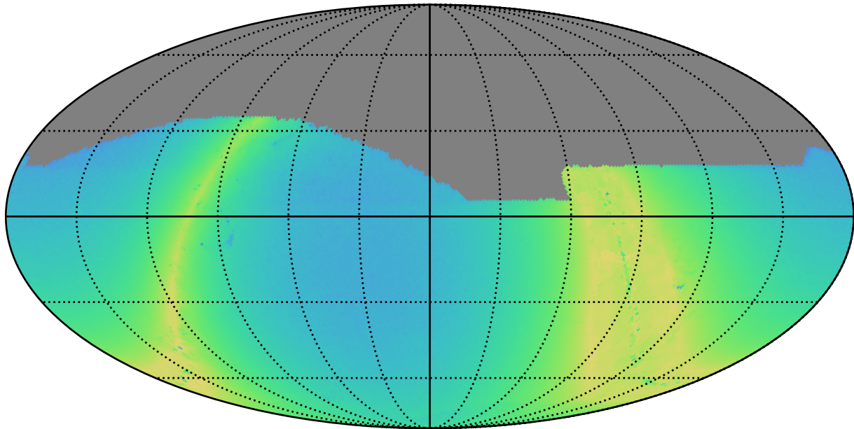
extra_ss_neo4_v3.4_10yrs z: N stars to Precision 0.20
