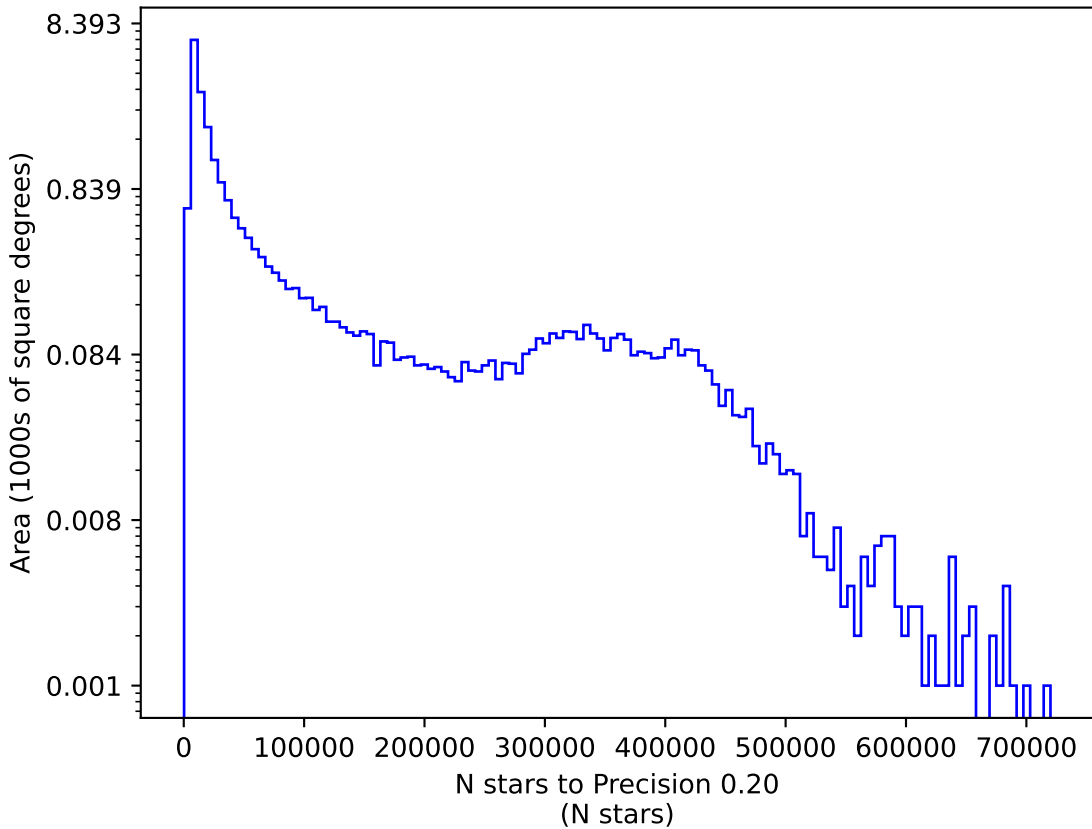
extra_ss_neo4_v3.4_10yrs y: N stars to Precision 0.20
