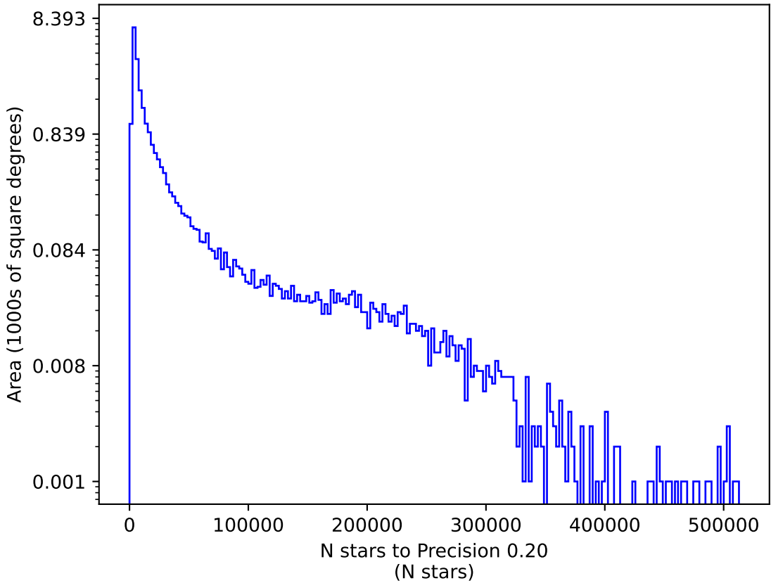
extra_ss_neo4_v3.4_10yrs u: N stars to Precision 0.20
