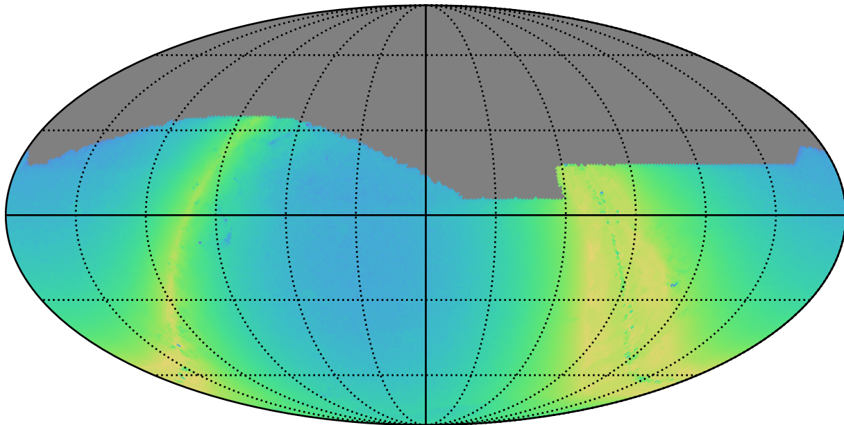
extra_ss_neo4_v3.4_10yrs r: N stars to Precision 0.20
