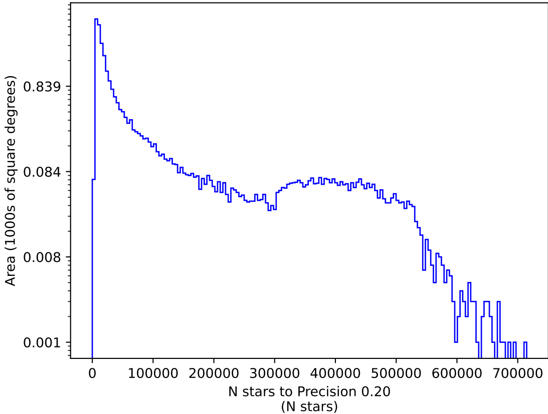
extra_ss_neo4_v3.4_10yrs r: N stars to Precision 0.20
