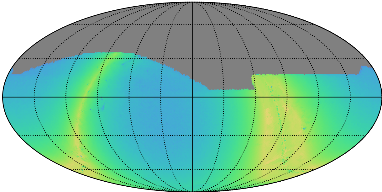
extra_ss_neo4_v3.4_10yrs i: N stars to Precision 0.20
