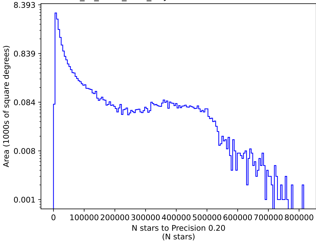
extra_ss_neo4_v3.4_10yrs i: N stars to Precision 0.20
