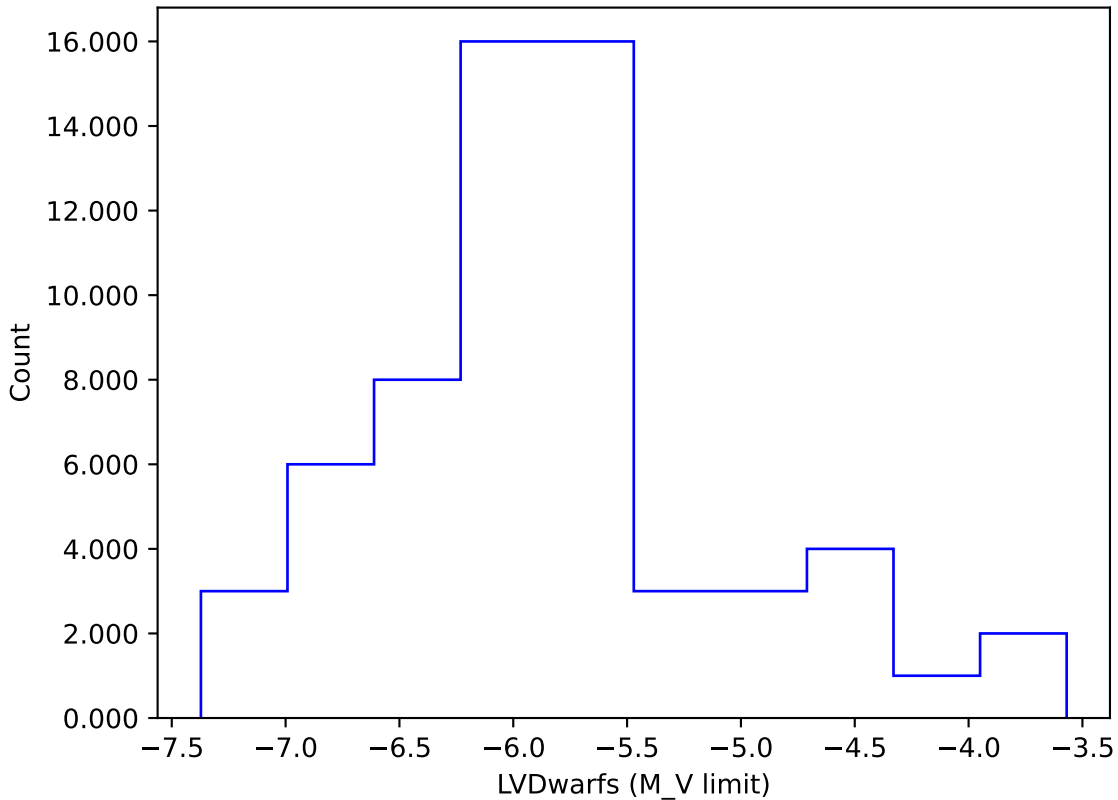
extra_ss_neo4_v3.4_10yrs gi: LVDwarfs
