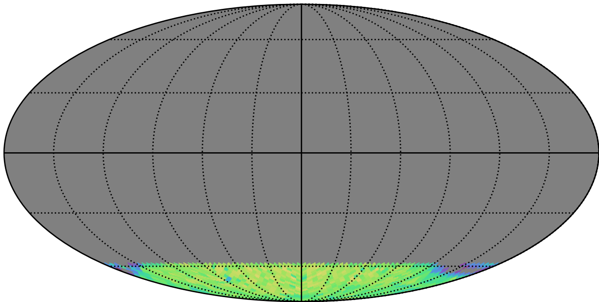
extra_ss_neo4_v3.4_10yrs gi SCP: LVDwarfs
