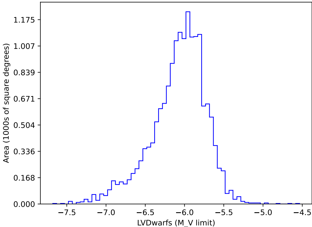
extra_ss_neo4_v3.4_10yrs gi: LVDwarfs
