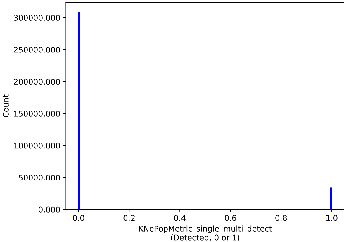
extra_ss_neo4_v3.4_10yrs single model: KNePopMetric_single_multi_detect
