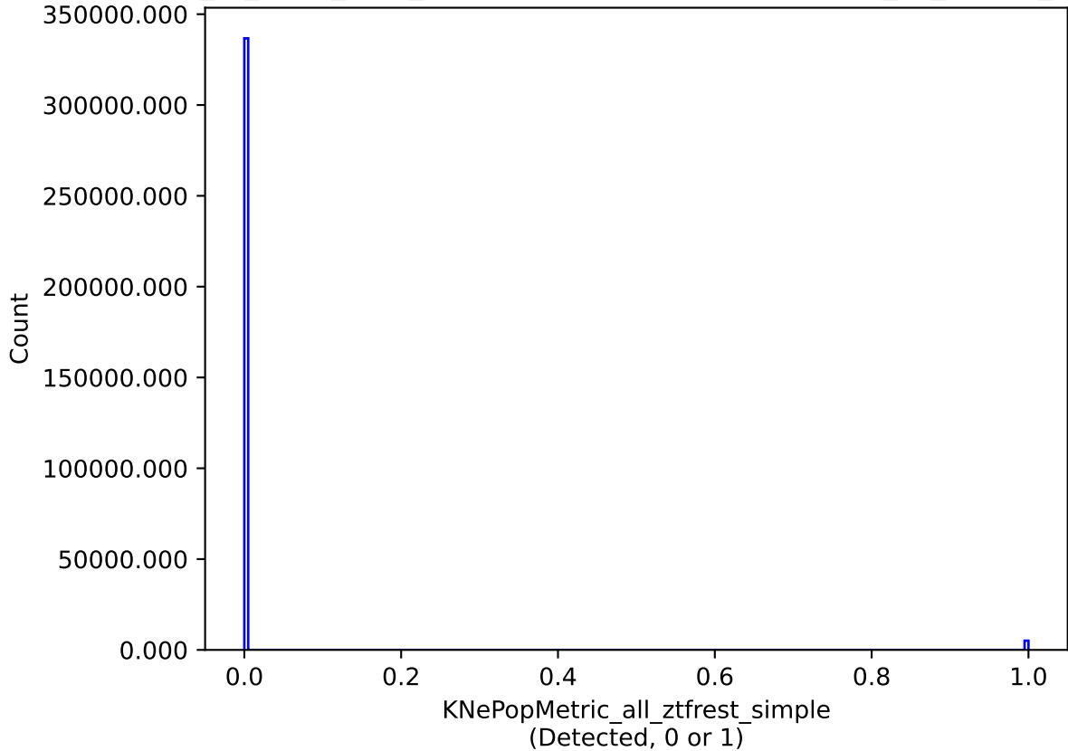
extra_ss_neo4_v3.4_10yrs all models: KNePopMetric_all_ztfrest_simple
