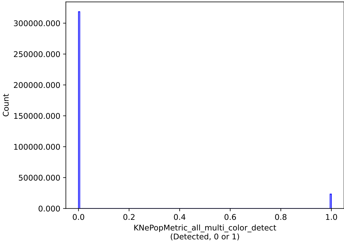
extra_ss_neo4_v3.4_10yrs all models: KNePopMetric_all_multi_color_detect
