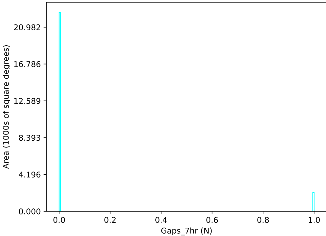
extra_ss_neo4_v3.4_10yrs u band: Gaps_7hr
