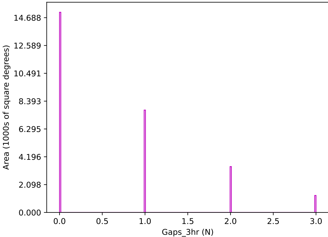
extra_ss_neo4_v3.4_10yrs z band: Gaps_3hr
