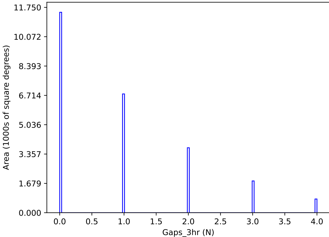
extra_ss_neo4_v3.4_10yrs y band: Gaps_3hr
