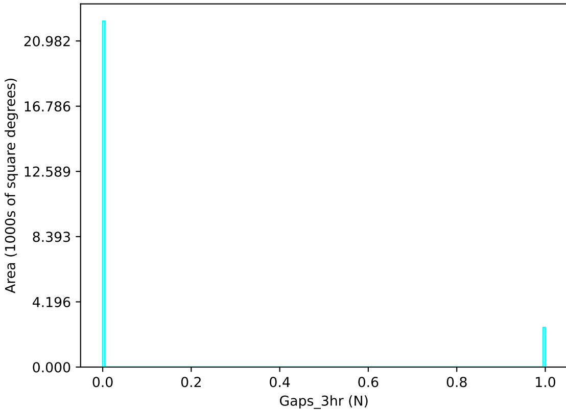
extra_ss_neo4_v3.4_10yrs u band: Gaps_3hr
