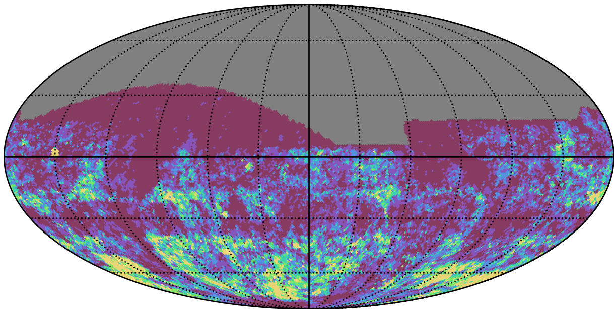
extra_ss_neo4_v3.4_10yrs r band: Gaps_3hr
