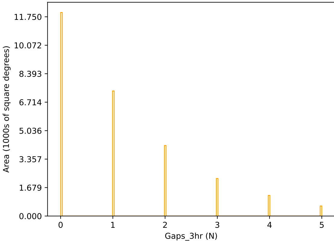
extra_ss_neo4_v3.4_10yrs r band: Gaps_3hr
