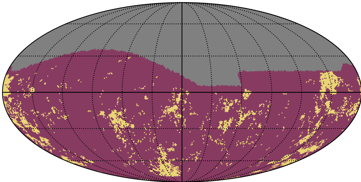
extra_ss_neo4_v3.4_10yrs g band: Gaps_3hr
