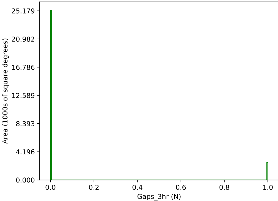
extra_ss_neo4_v3.4_10yrs g band: Gaps_3hr
