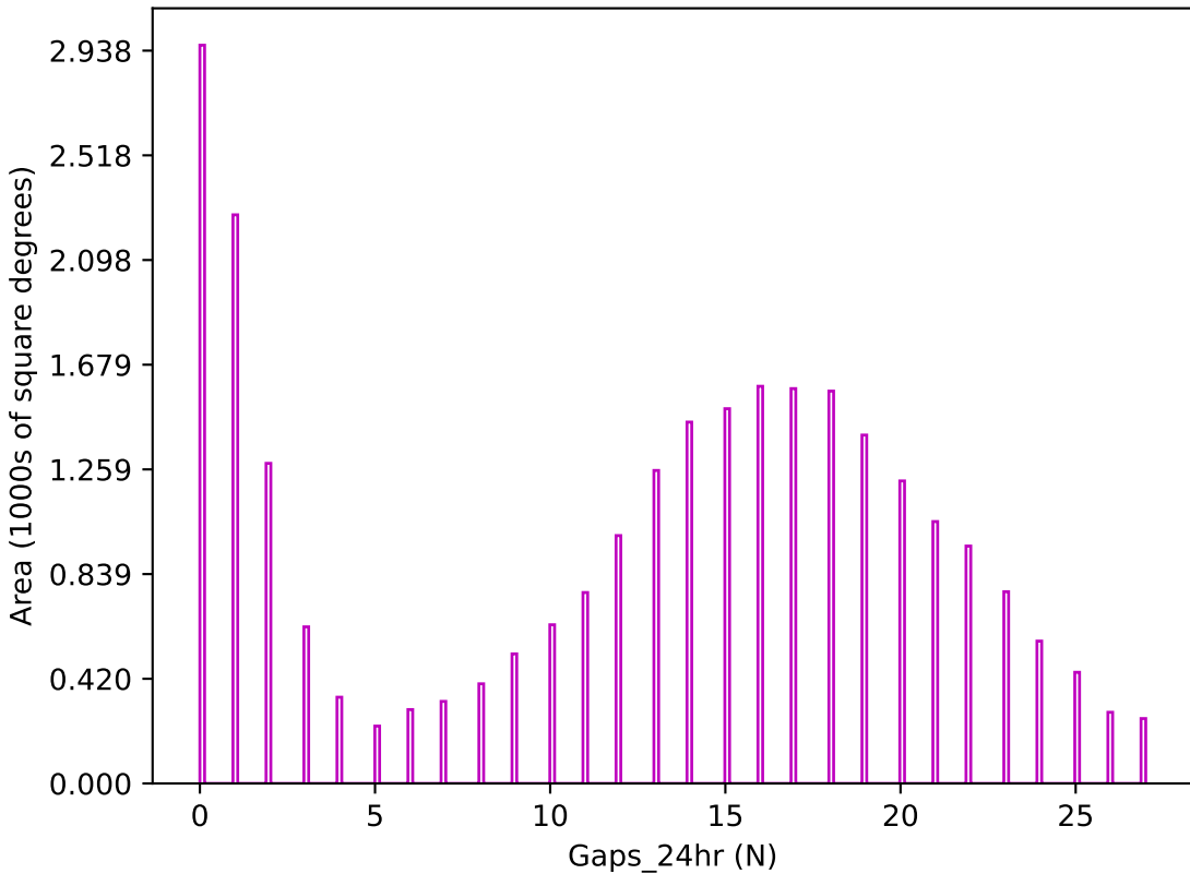
extra_ss_neo4_v3.4_10yrs z band: Gaps_24hr
