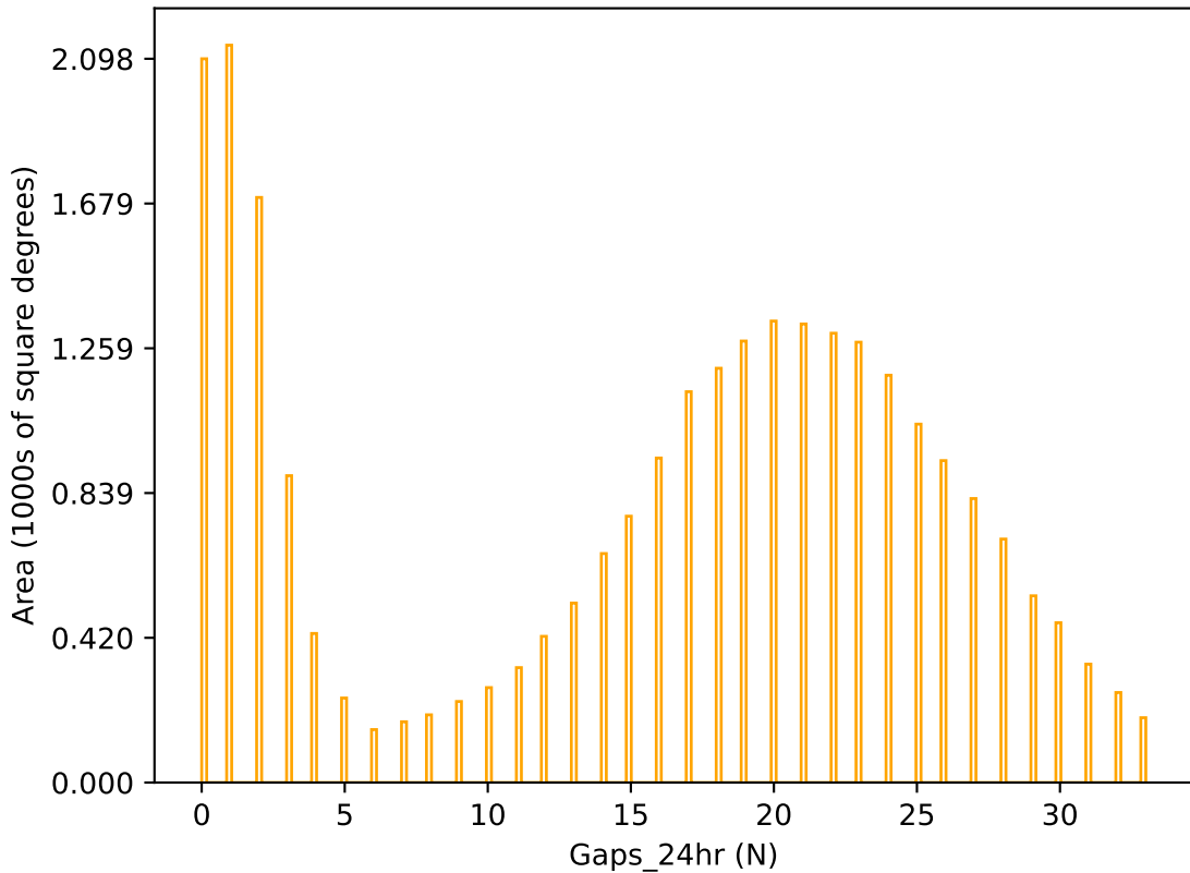
extra_ss_neo4_v3.4_10yrs r band: Gaps_24hr
