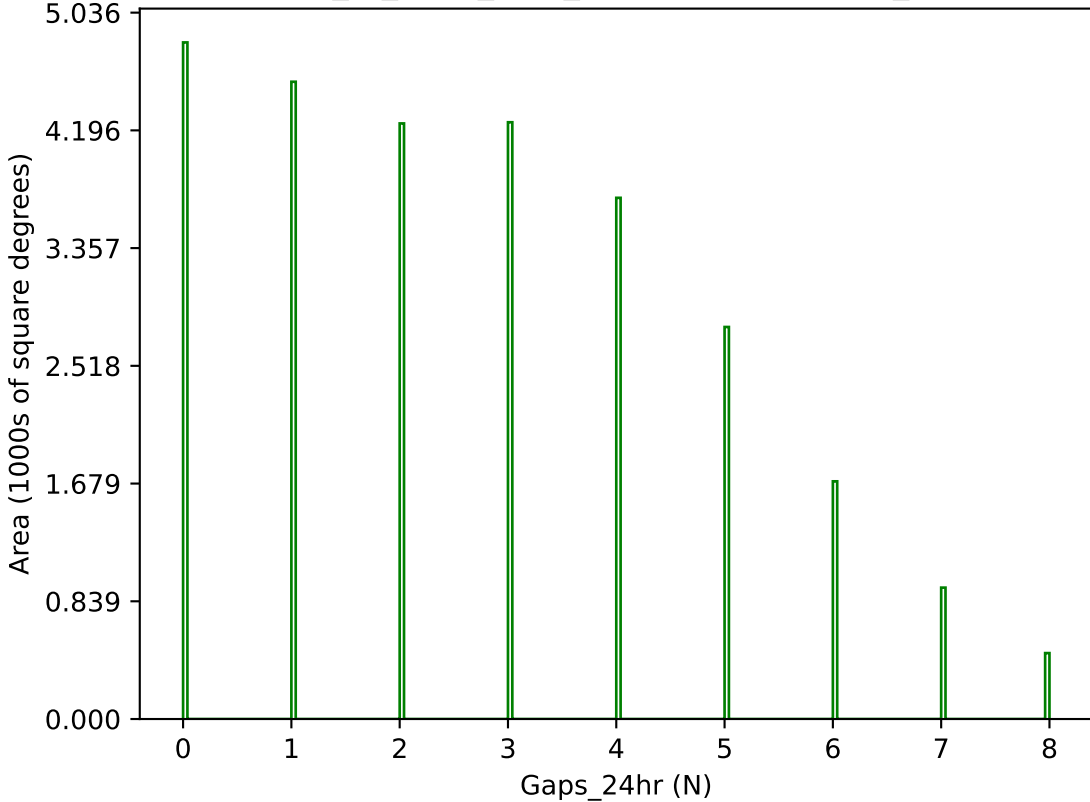
extra_ss_neo4_v3.4_10yrs g band: Gaps_24hr
