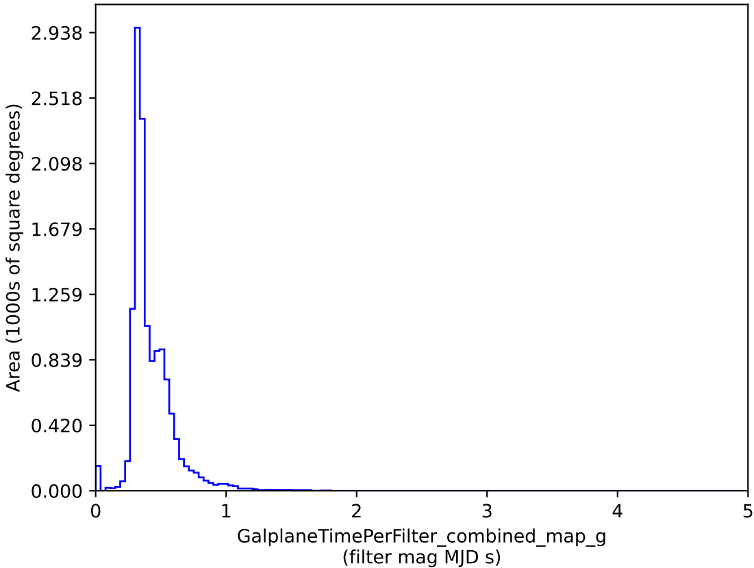
extra_ss_neo4_v3.4_10yrs : GalplaneTimePerFilter_combined_map_g
