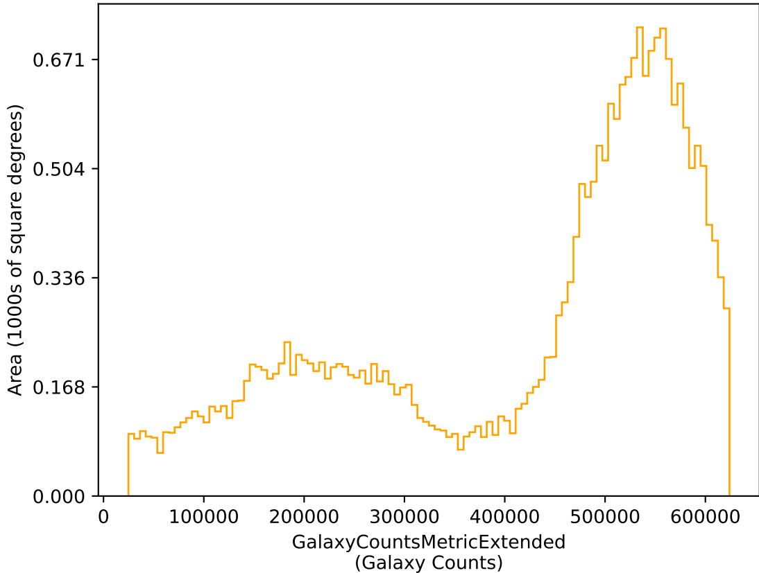
extra_ss_neo4_v3.4_10yrs r: GalaxyCountsMetricExtended
